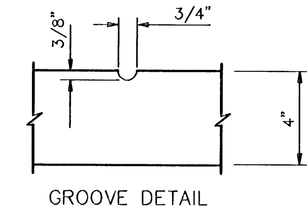
GROOVE DETAIL
