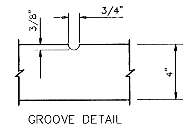
GROOVE DETAIL
