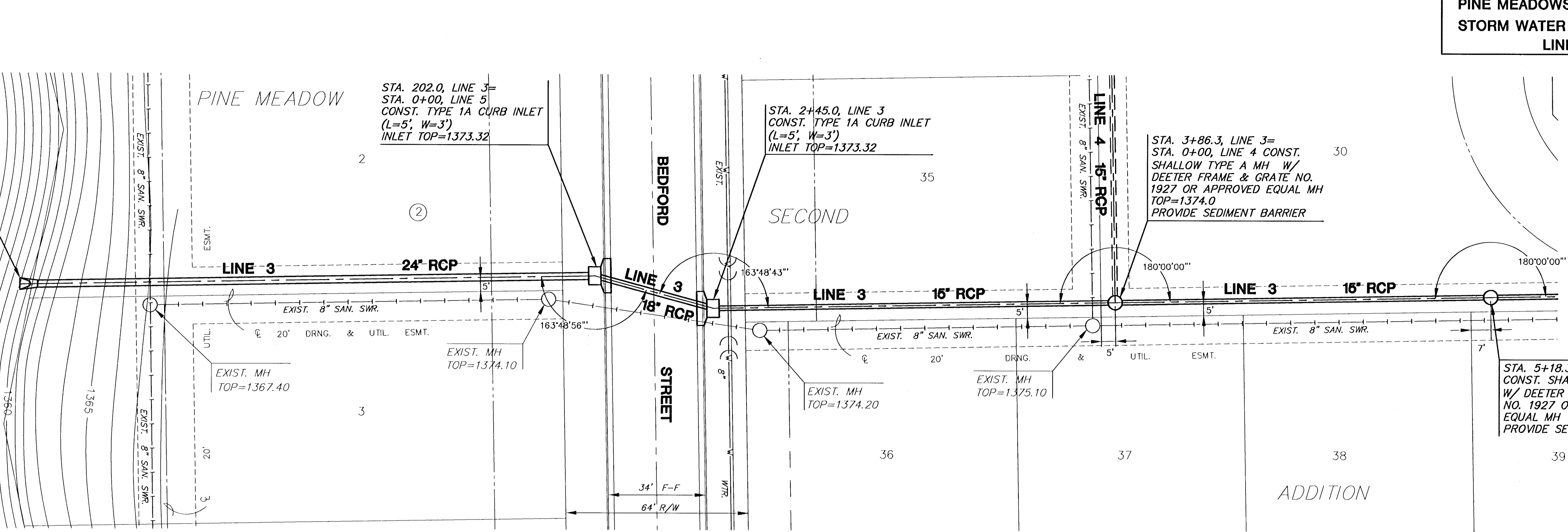
PLAN LINE 3 SCALE: 1"=20'
