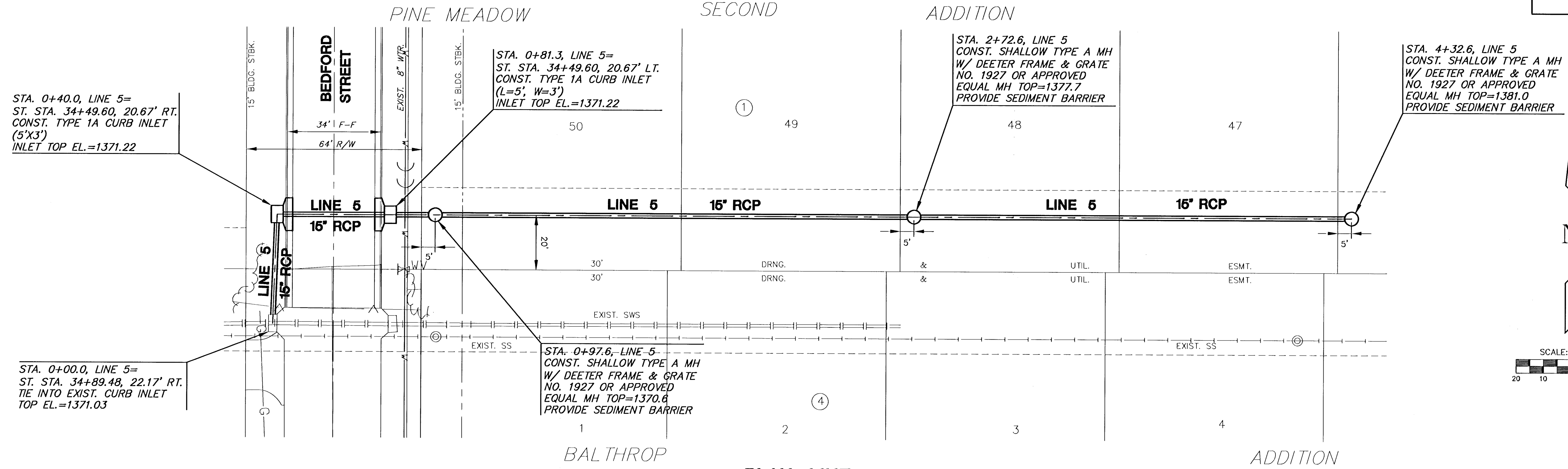
PLAN LINE 5 SCALE: 1"=20'
