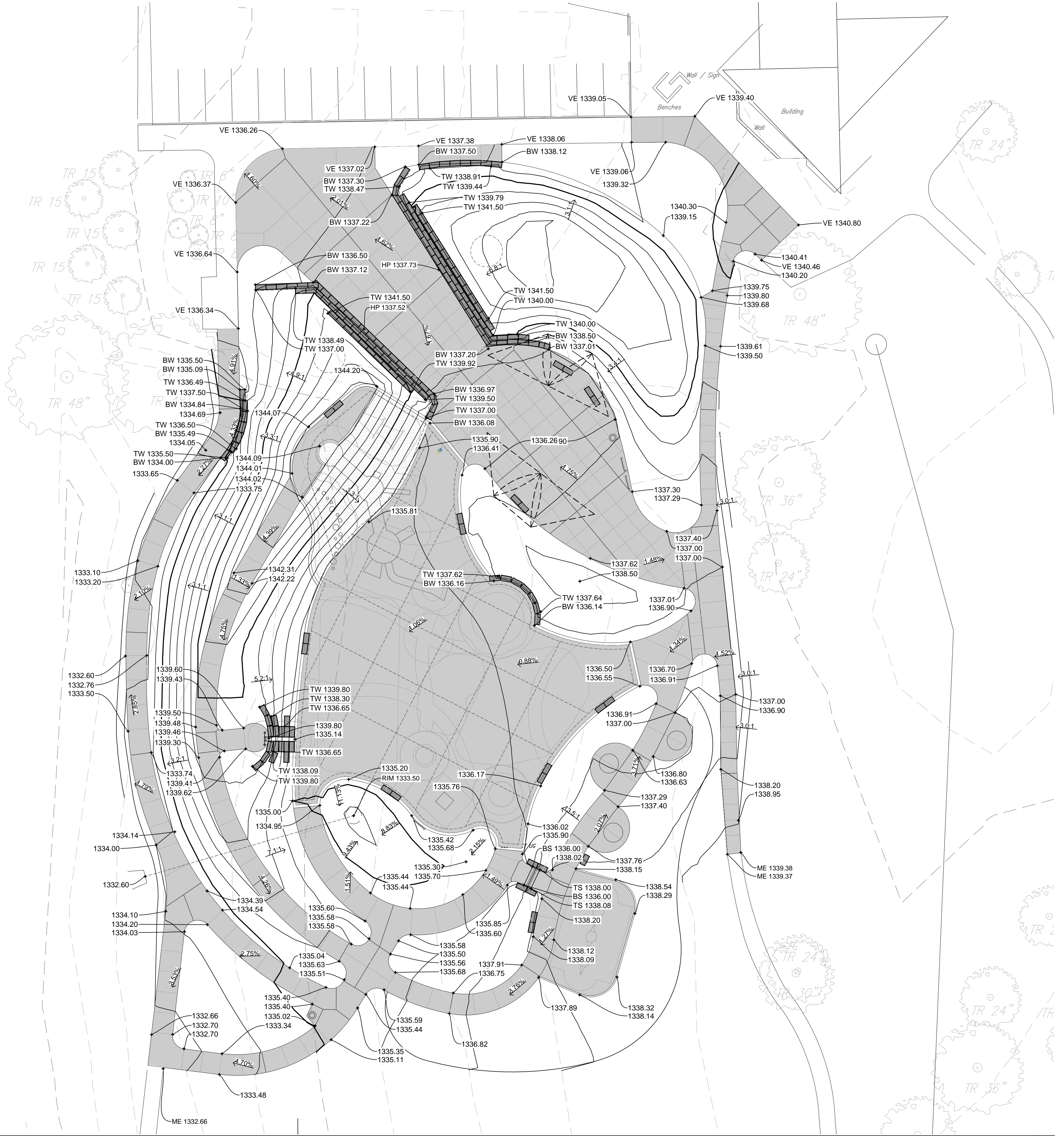
01 GRADING PLAN ENLARGEMENT
