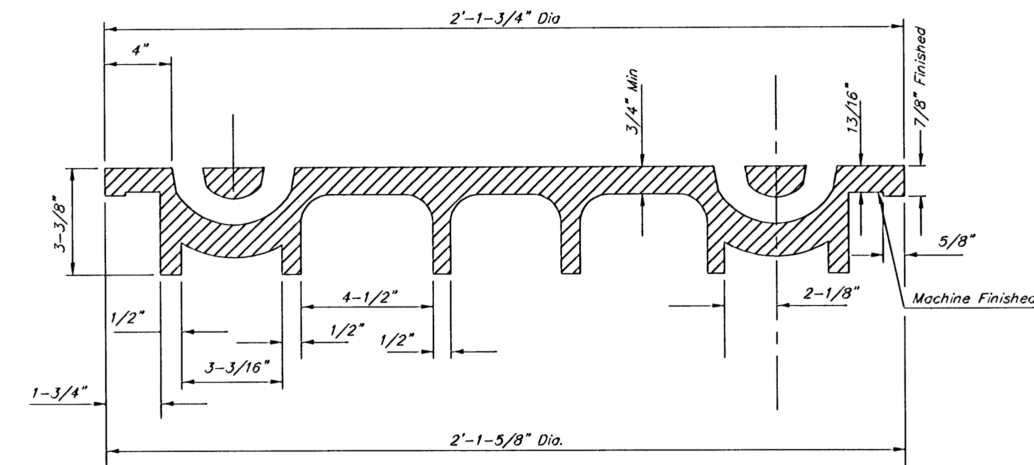
SECTION VIEW
