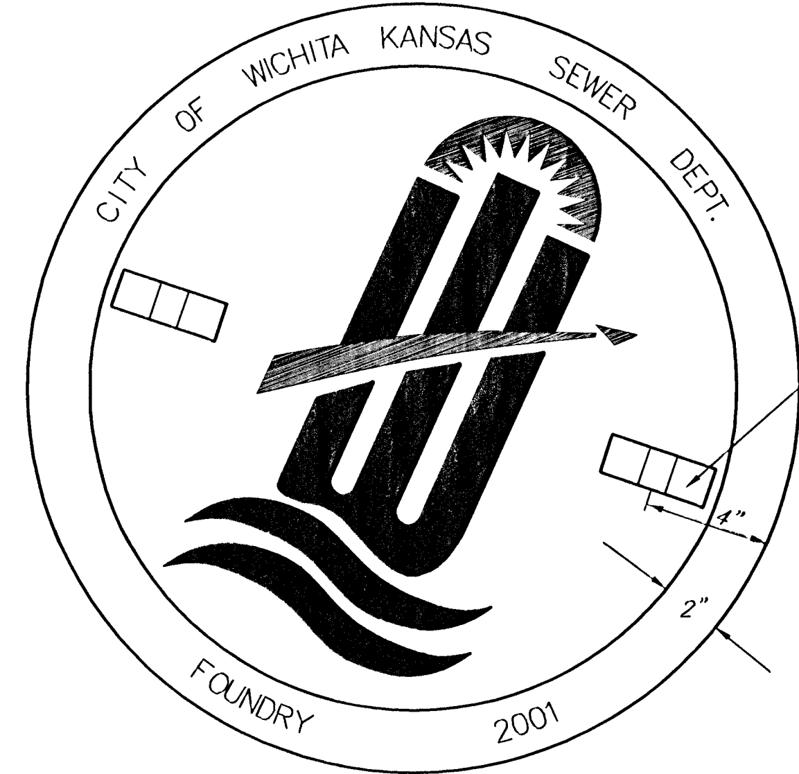
TOP VIEW
