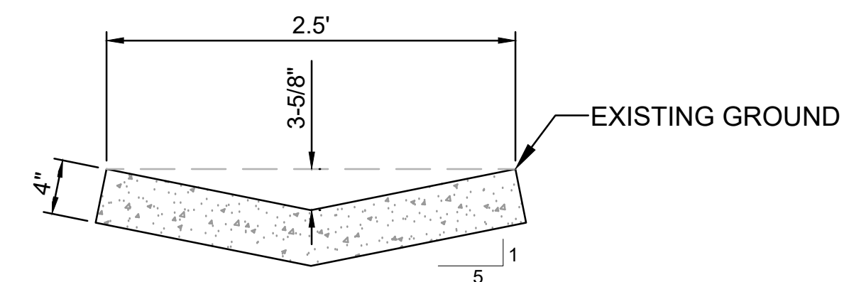
CONCRETE FLUME CROSS-SECTION NOT TO SCALE
