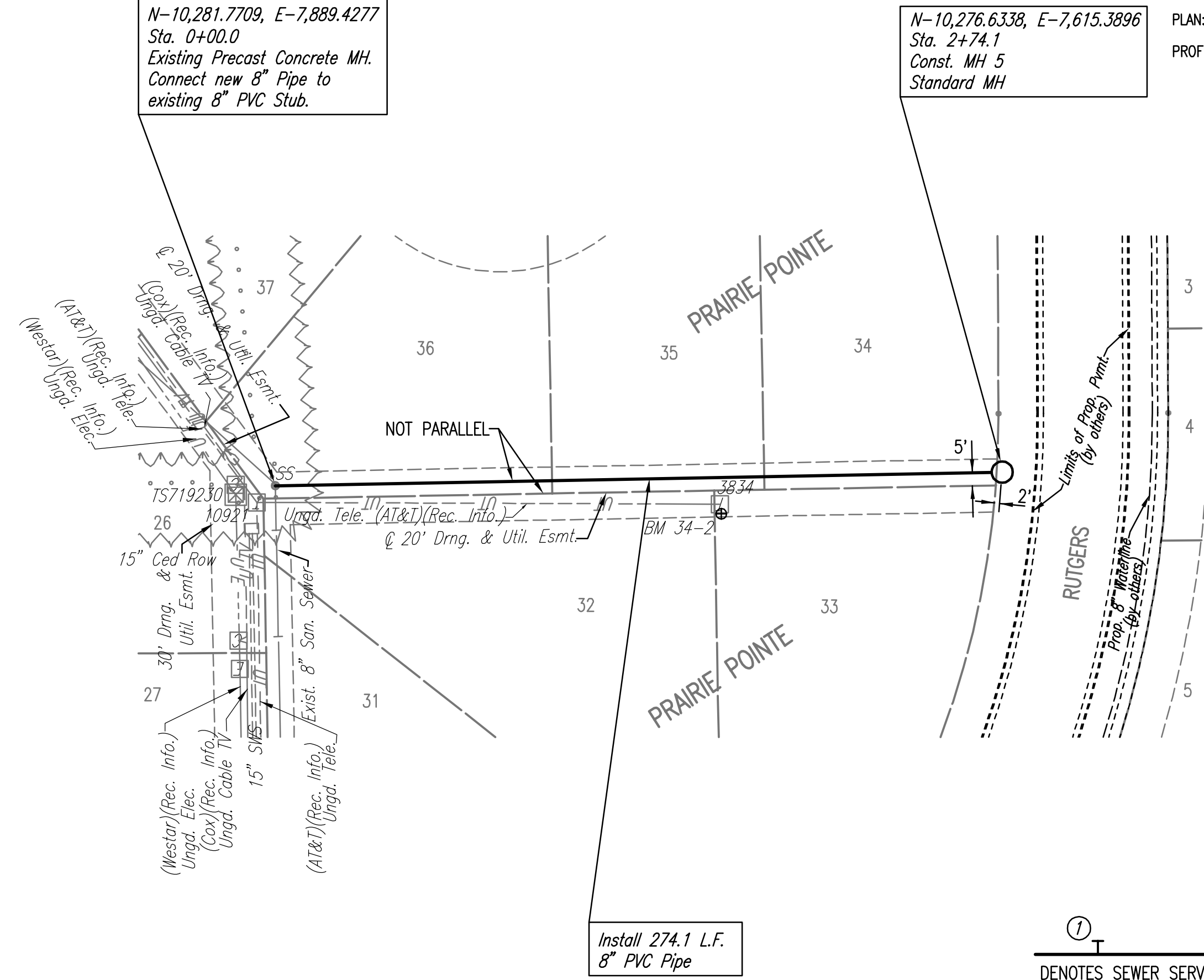
SANITARY SEWER LINE NO. 2
