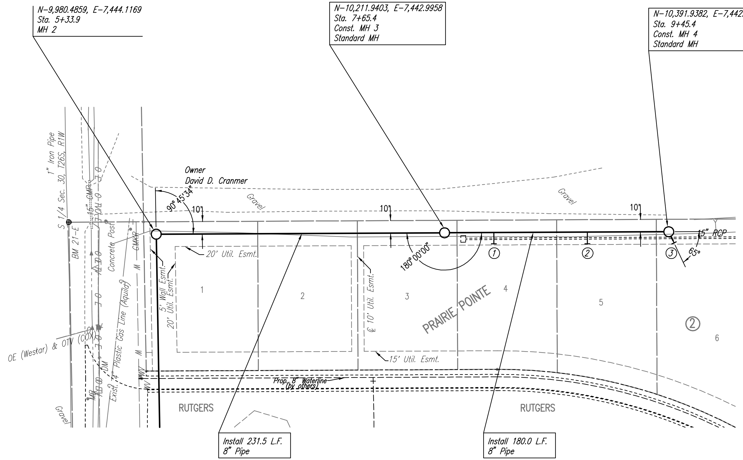
SANITARY SEWER LINE NO. 1
