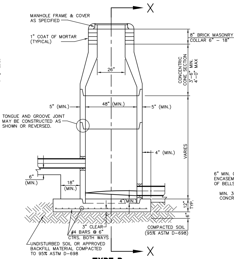
TYPE P INSIDE DROP MANHOLE
