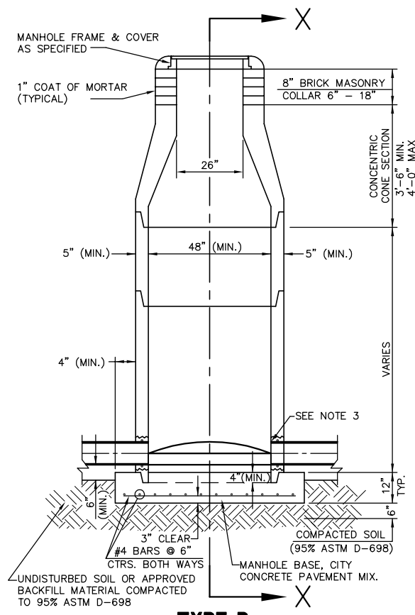
TYPE P STANDARD MANHOLE
