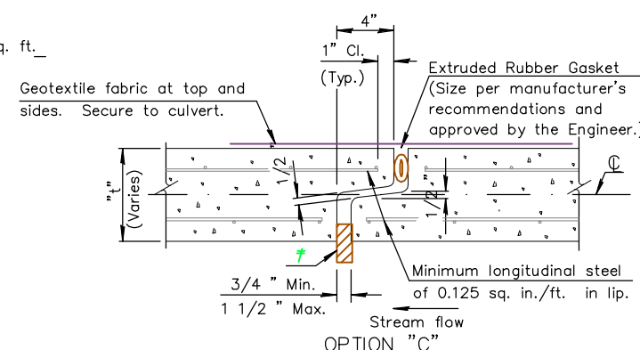
OPEN JOINT DETAIL
