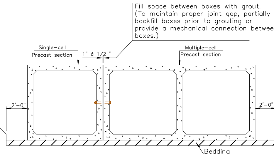
TYPICAL INSTALLATION DETAILS
