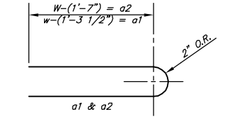
BENDING DIAGRAM
