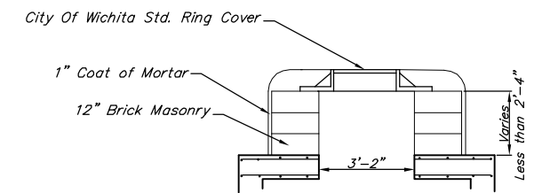
MANHOLE STACK LESS THAN 2.33'
