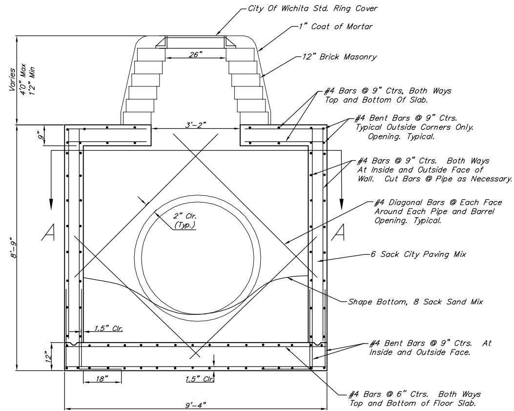
REINFORCED CONCRETE MANHOLE Sta. 12+00.00, SWS Line 1 (Looking South)
