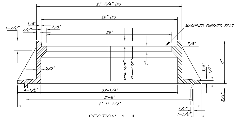
SECTION A-A STANDARD MANHOLE FRAME Weight = 250 Lbs.
