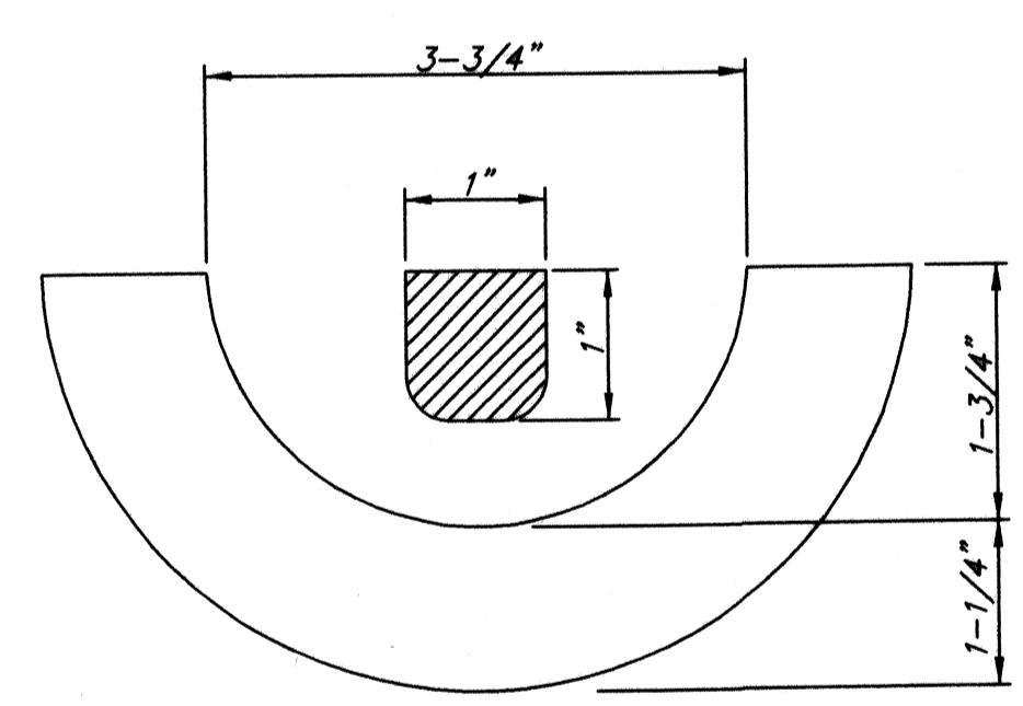
SECTION VIEW
