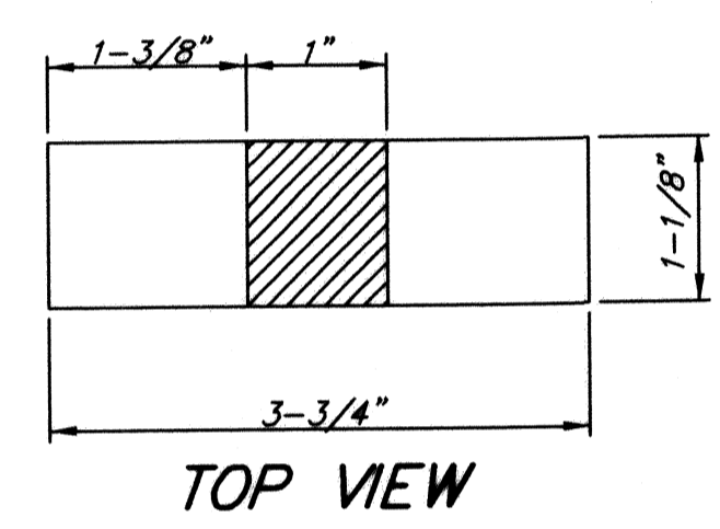
PICKHOLE DETAIL
