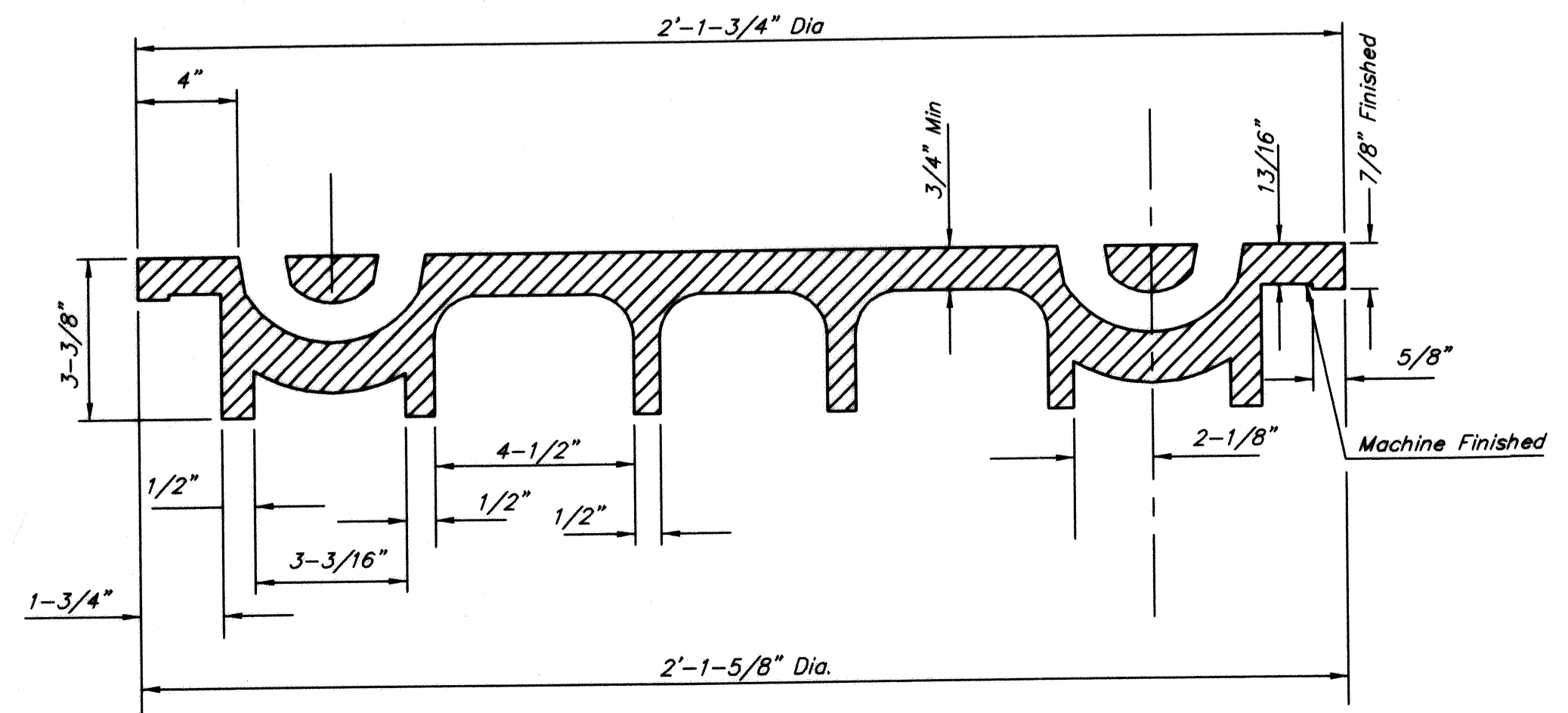
SECTION VIEW
