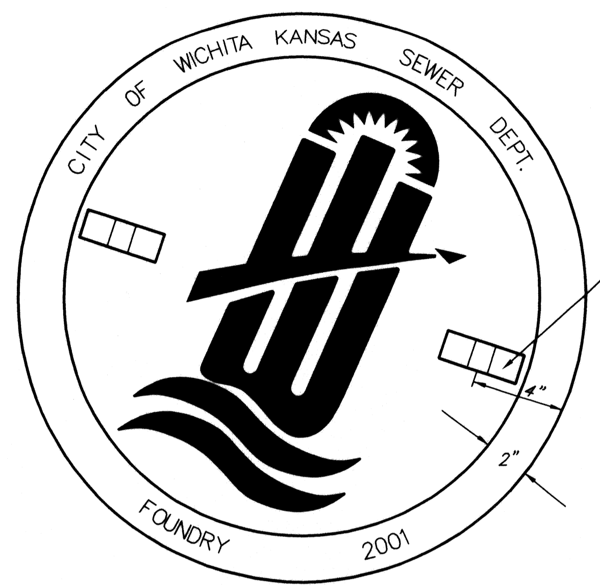
TOP VIEW
