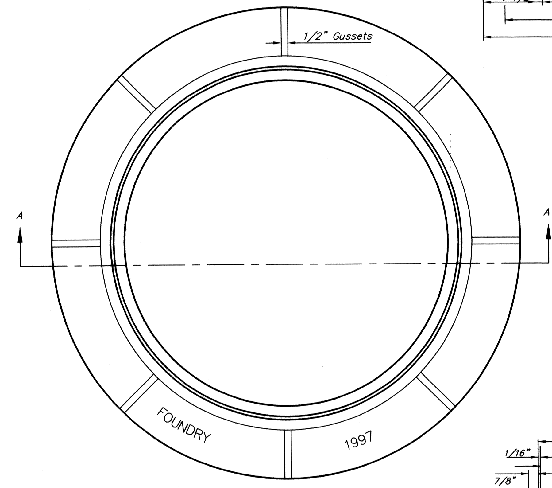
TOP VIEW
