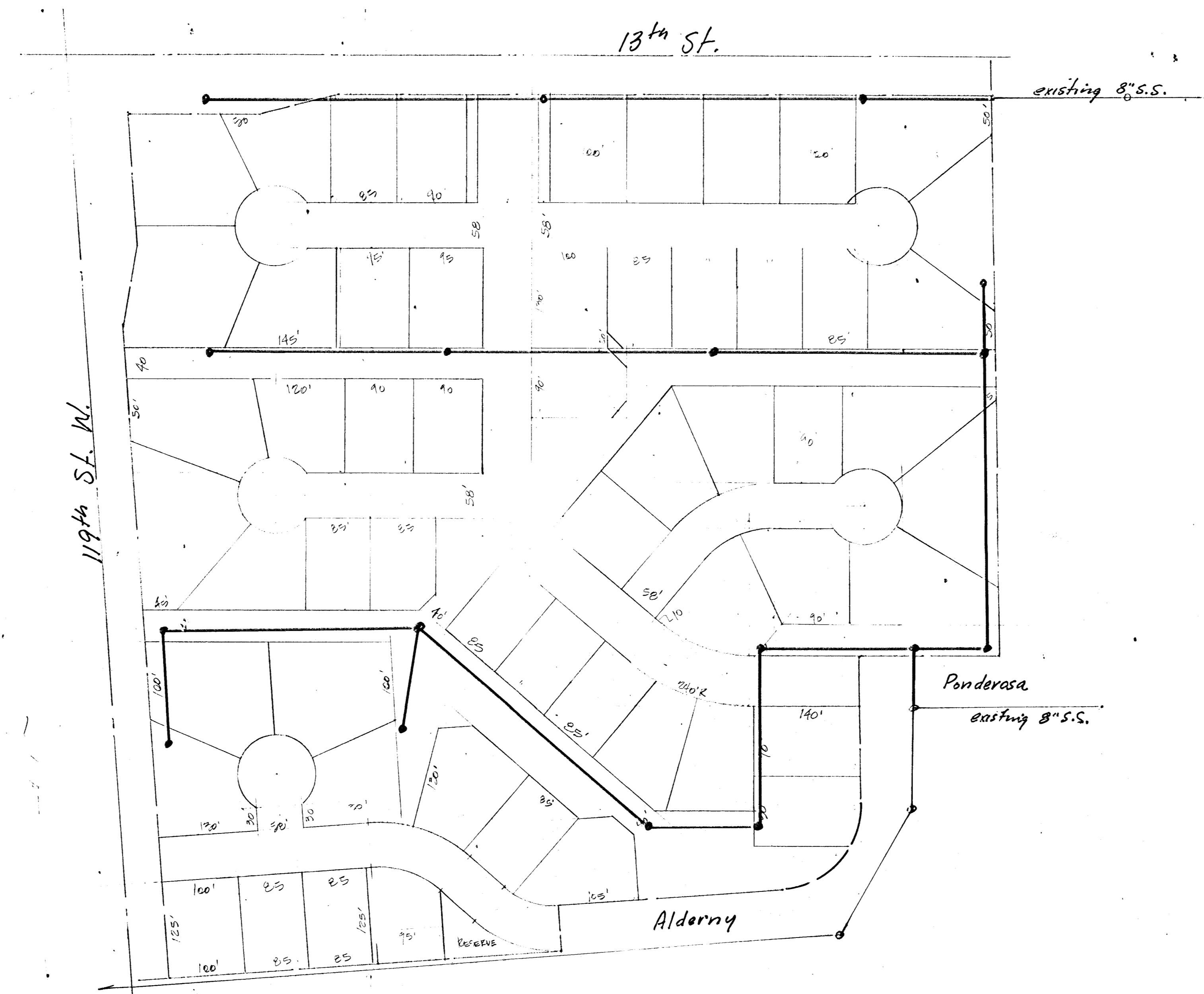
Sanitary Sewer Layout Briarwood 5 th Addn.
