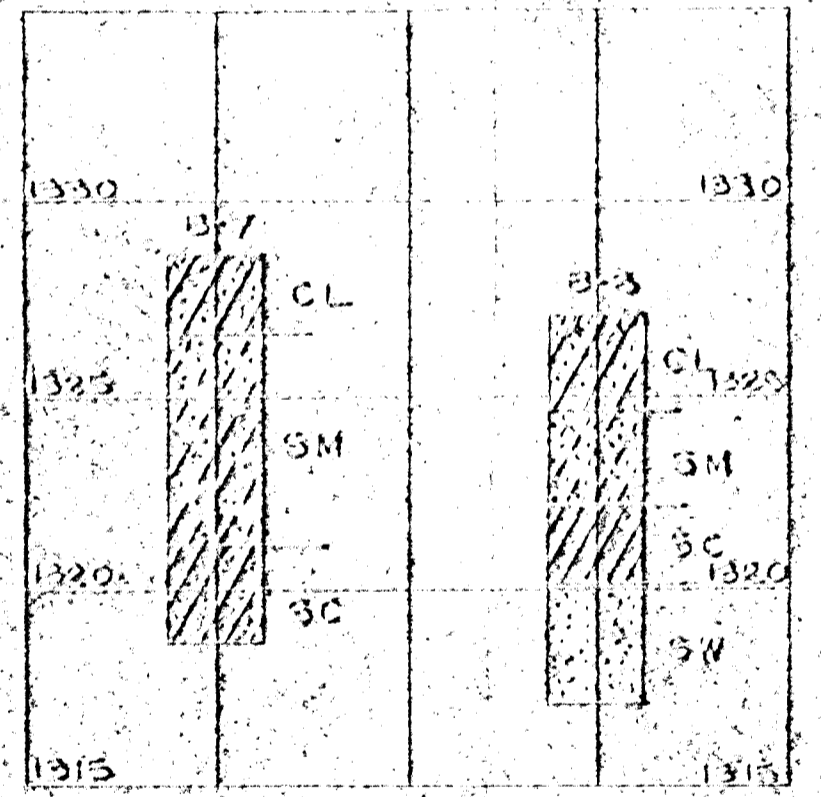
BORING LOG B-7 & B-3
