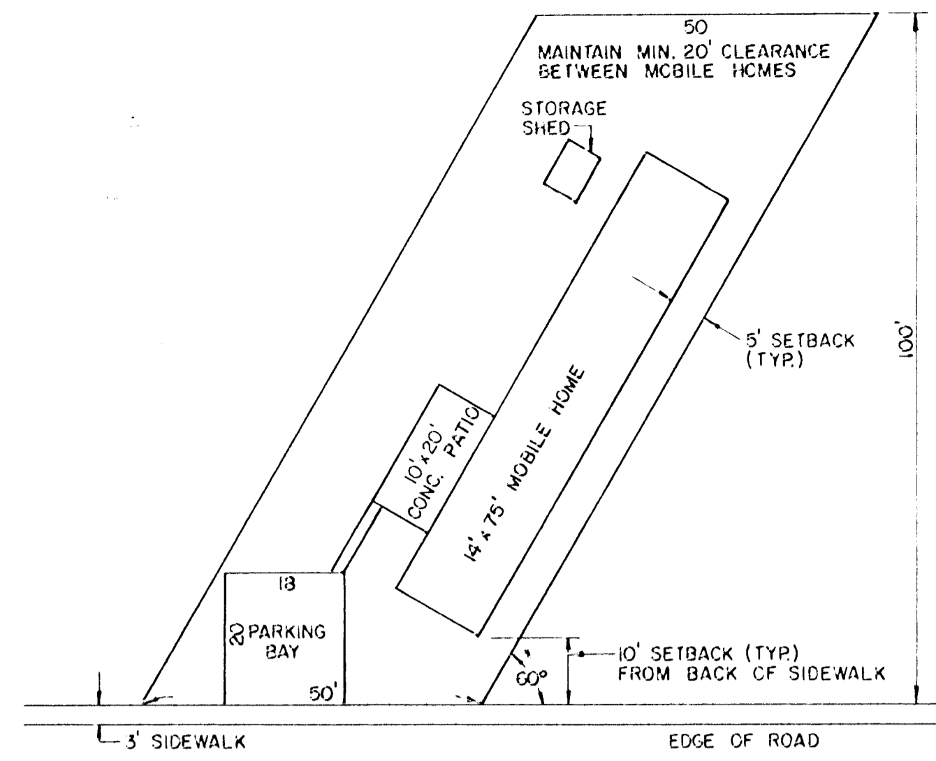
TYPICAL SITE LAYOUT SCALE: 1" = 20'
