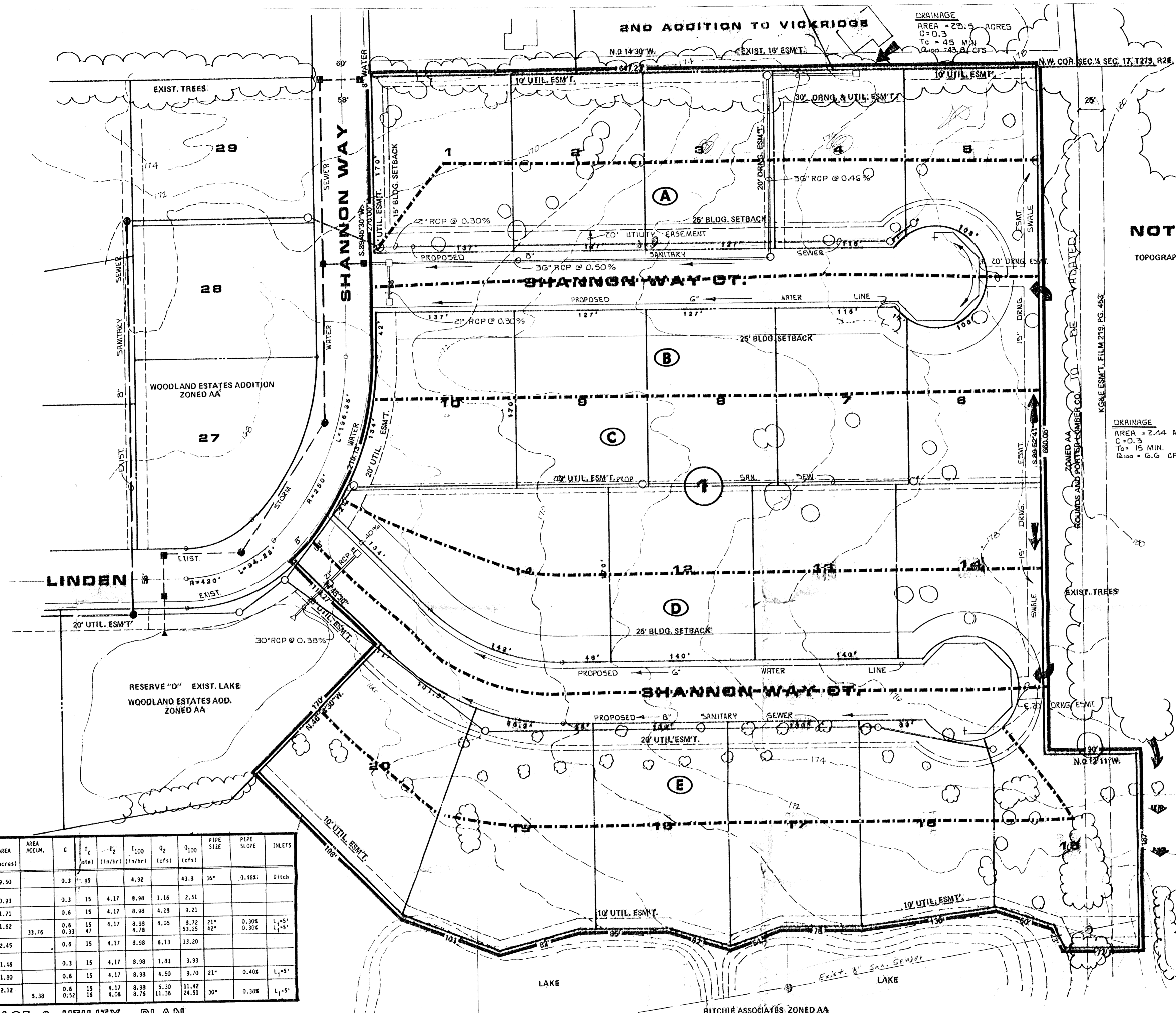
DRAINAGE & UTILITY PLAN
