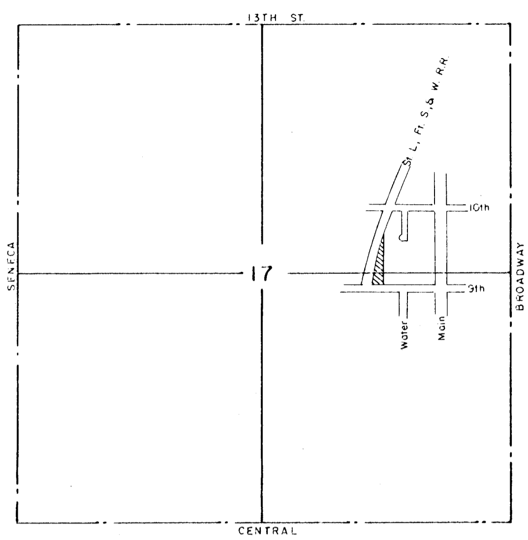
VICINITY MAP 1" = 1000'
