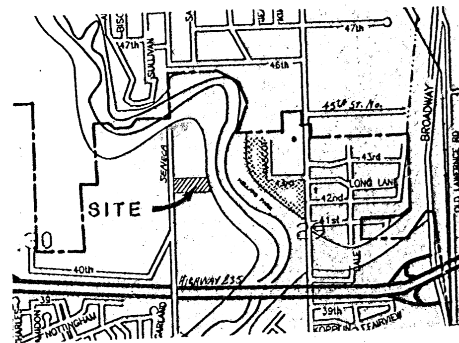
VICINITY MAP
