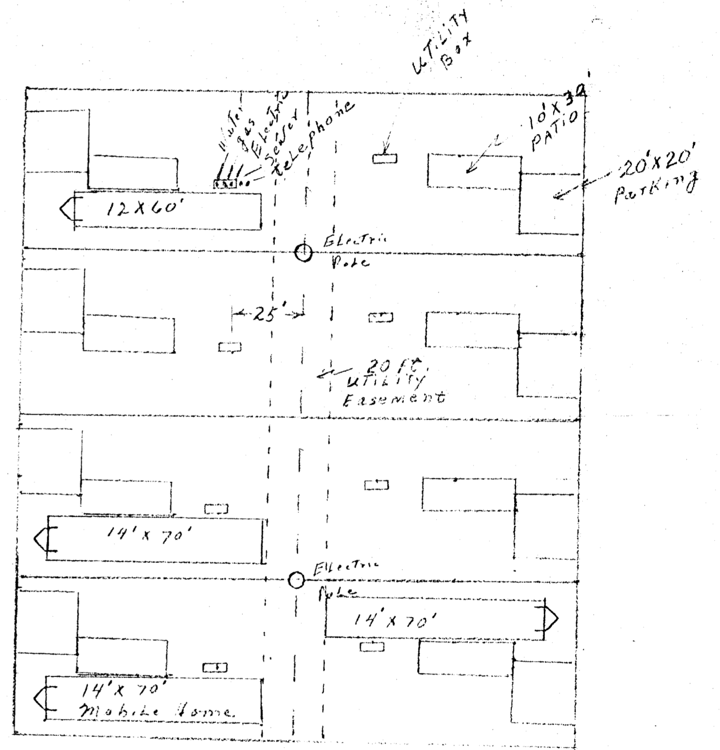
INDIVIDUAL site Layout
