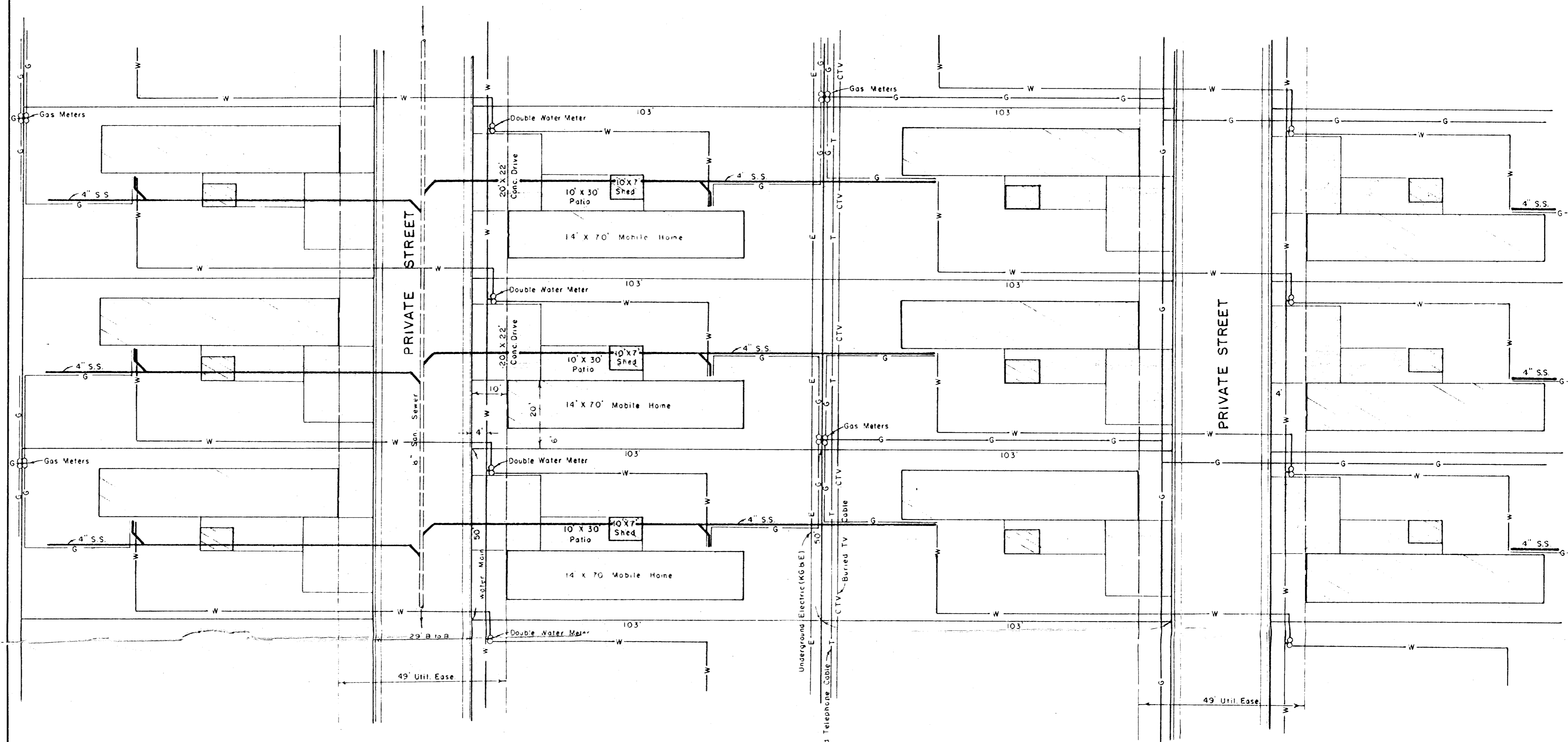
MOBILE MANOR SOUTH TYPICAL UTILITY LAYOUT
