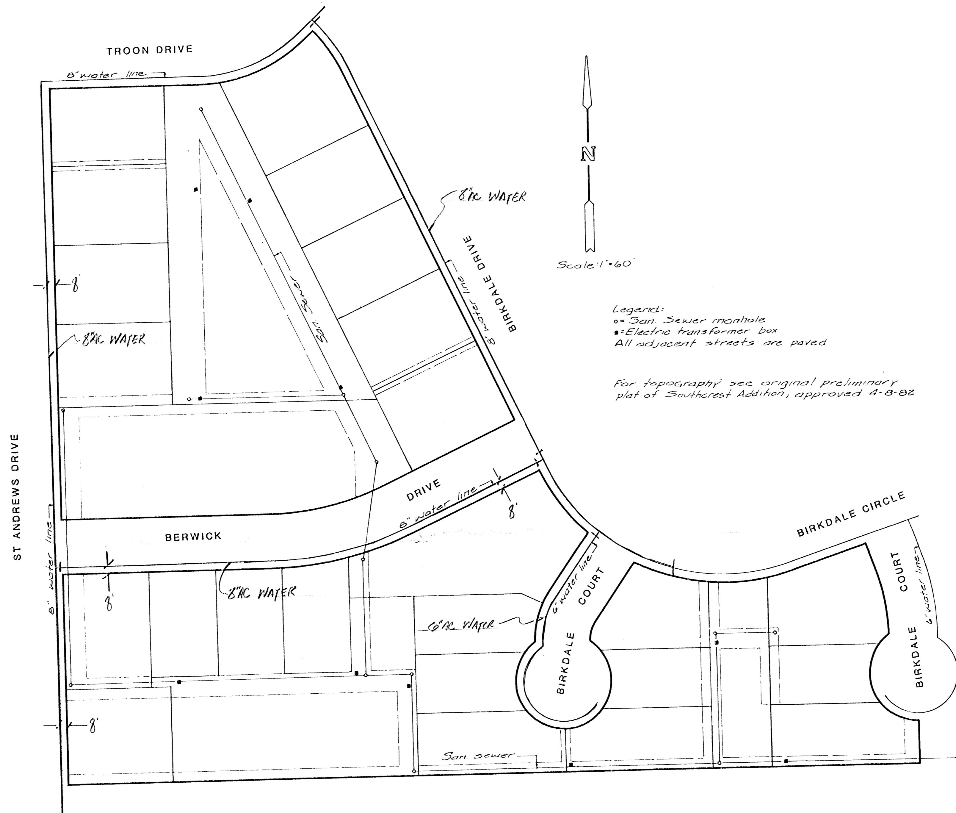
SKETCH PLAN & EXISTING UTILITY LOCATIONS CRESTVIEW COUNTRY CLUB ESTATES SOUTHCREST SECOND ADDITION SEDGWICK COUNTY, KANSAS
