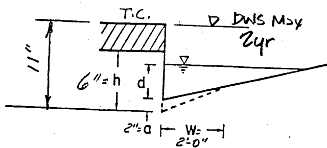
DEF. SKETCH, C.O.W. TYPE 1A INLET
