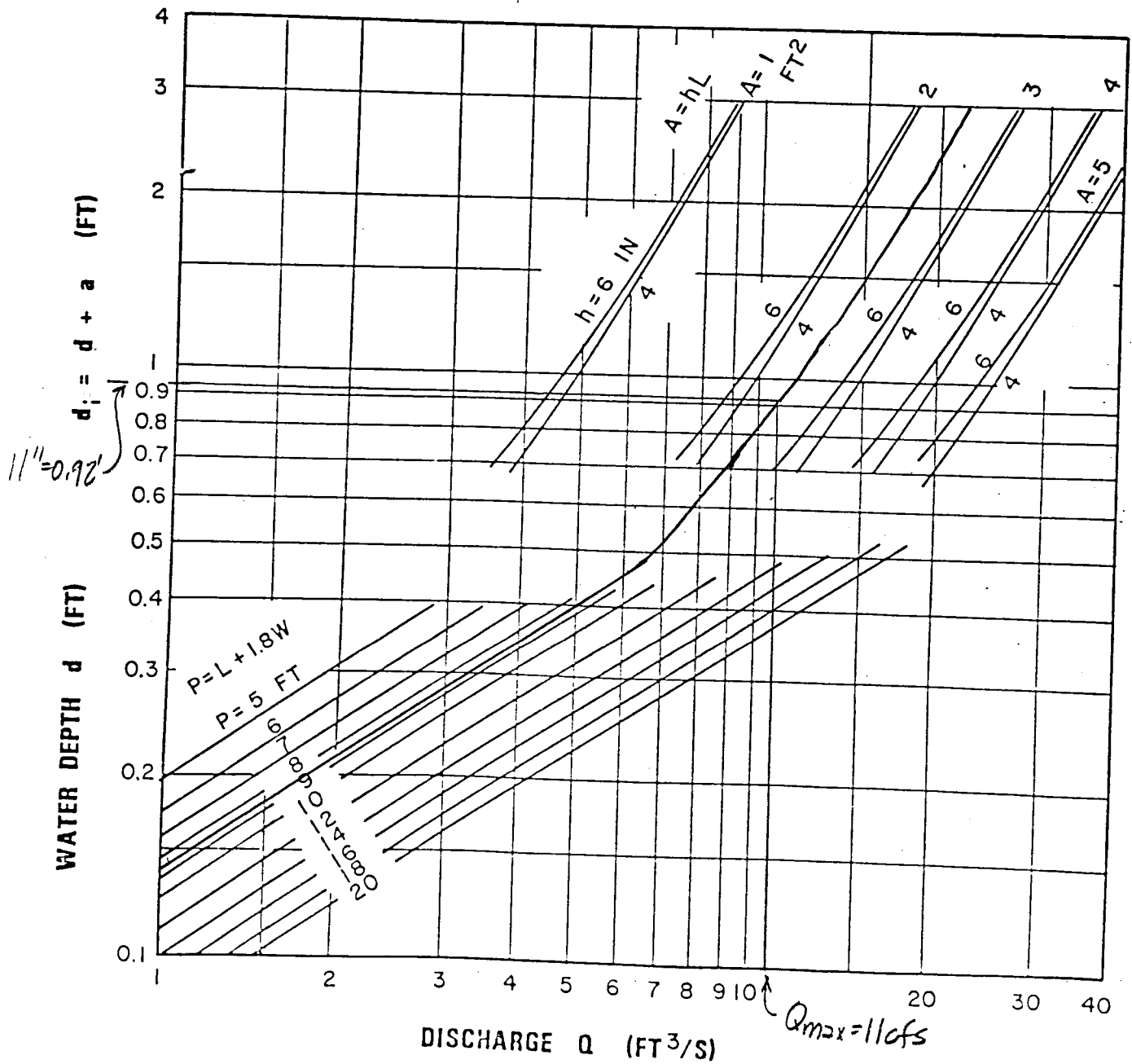
CHART 12. Depressed curb-opening inlet capacity in sump locations.
