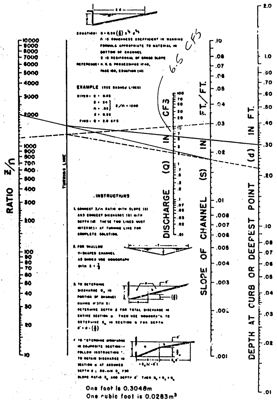
FIG. 5-1 (After FHWA)
