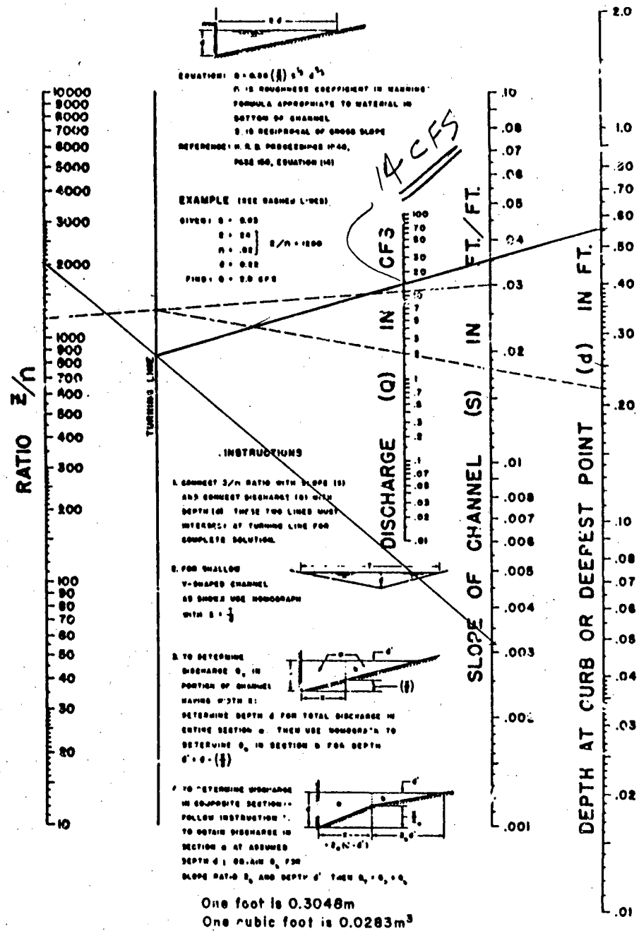
FIG. 5-1 (Adapted FHWA)
