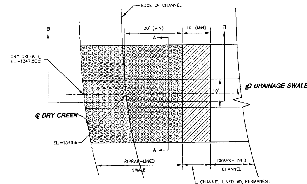
PLAN DRAINAGE SWALE OUTLET NOT TO SCALE
