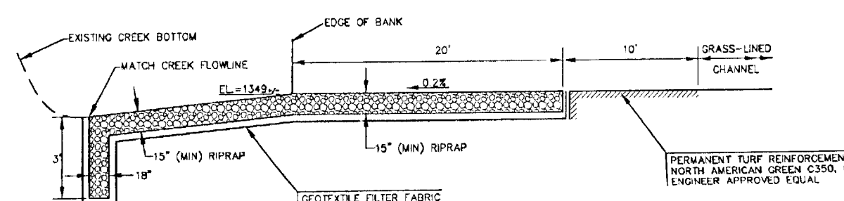
SECTION B-B DRAINAGE SWALE OUTLET NOT TO SCALE
