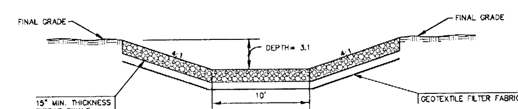
SECTION A-A DRAINAGE SWALE OUTLET NOT TO SCALE
