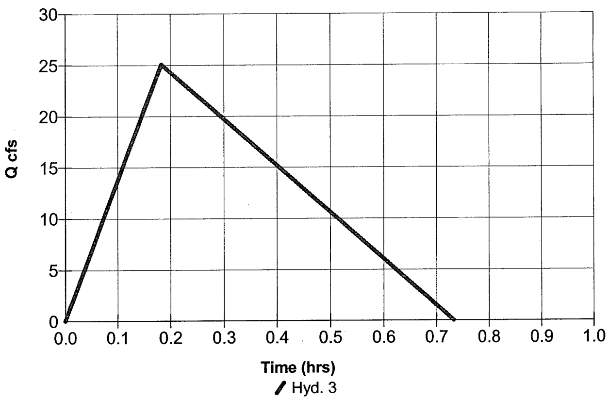
Hyd. No. 3 - Rational - 100 Yr - Q_p = 25.07 cfs - Sub-Basins B1, B3-B4
