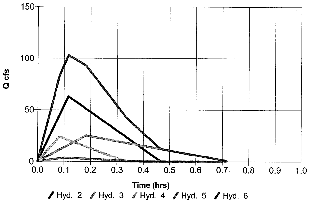
Hyd. No. 6 - Combine - 100 Yr - Qp = 103.04 cfs - Pond Inflows
