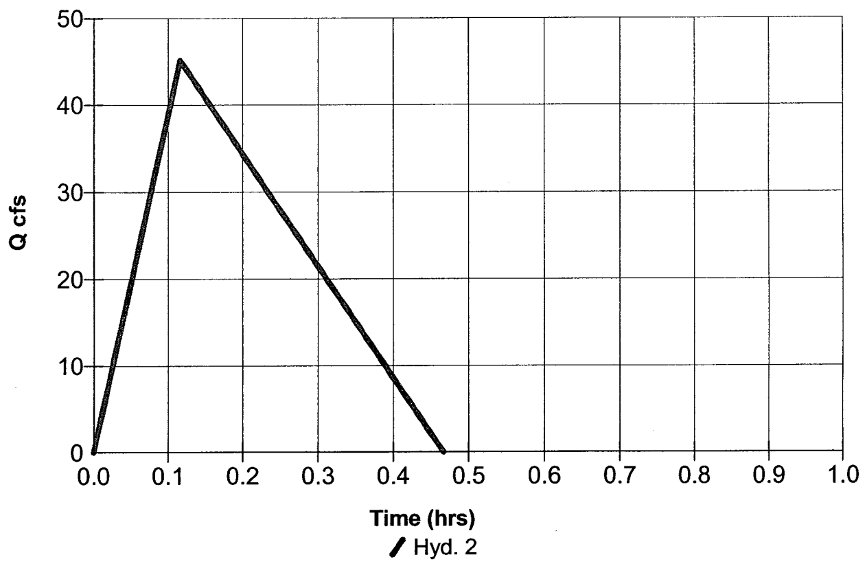
Hyd. No. 2 - Rational - 10 Yr - Qp = 45.14 cfs - Sub-Basins A1-A7
