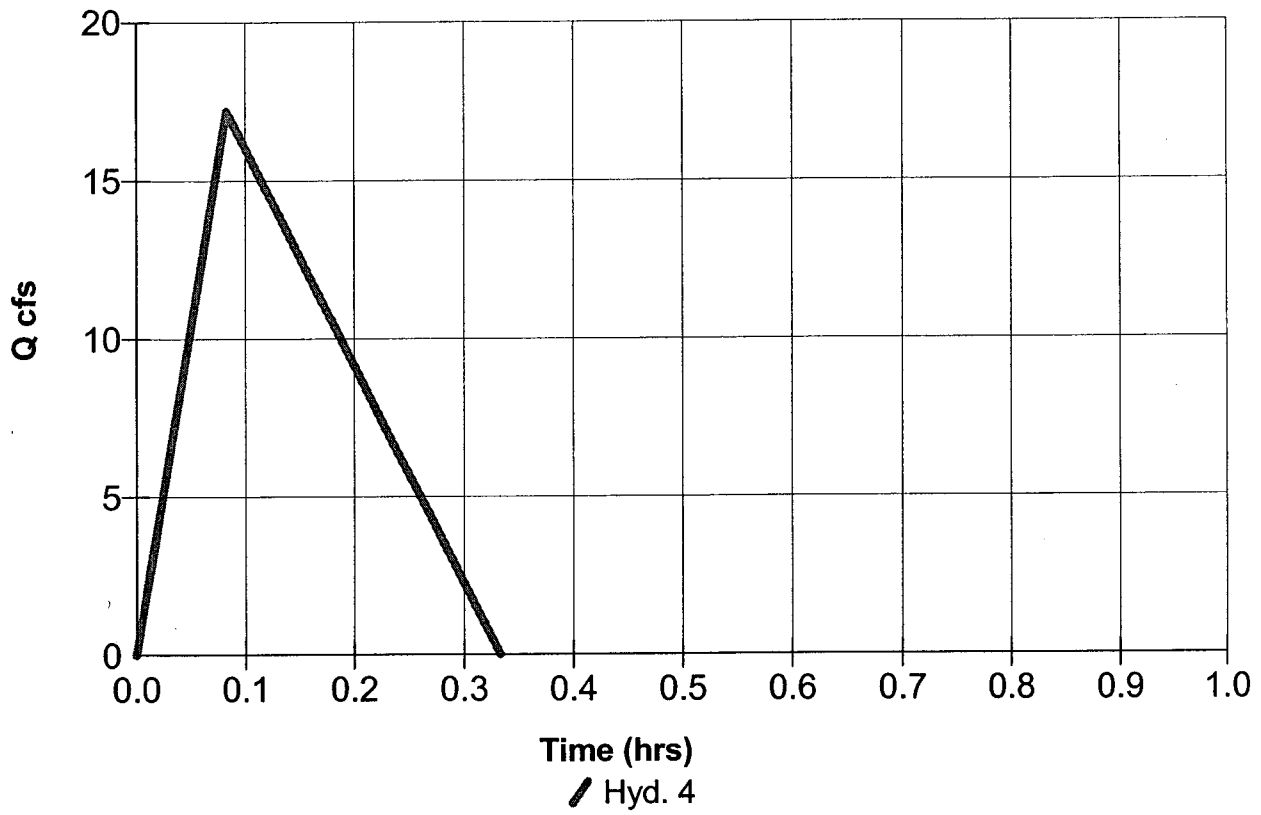
Hyd. No. 4 - Rational - 10 Yr - Qp = 17.18 cfs - Sub-basin B2
