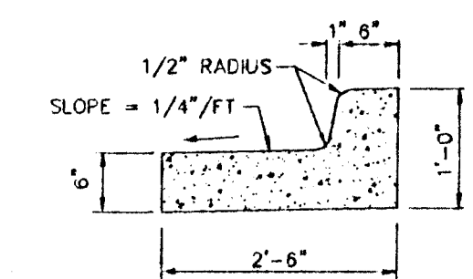
LOW EDGE CURB & GUTTER NOT TO SCALE
