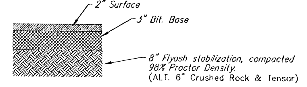
TYP. 5" ASPHALT PAVEMENT DETAIL NOT TO SCALE FOR THE PARKING LOT AREA
