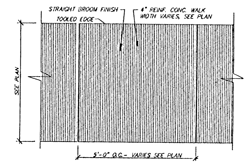
TYP. PATTERN IN WALK NOT TO SCALE
