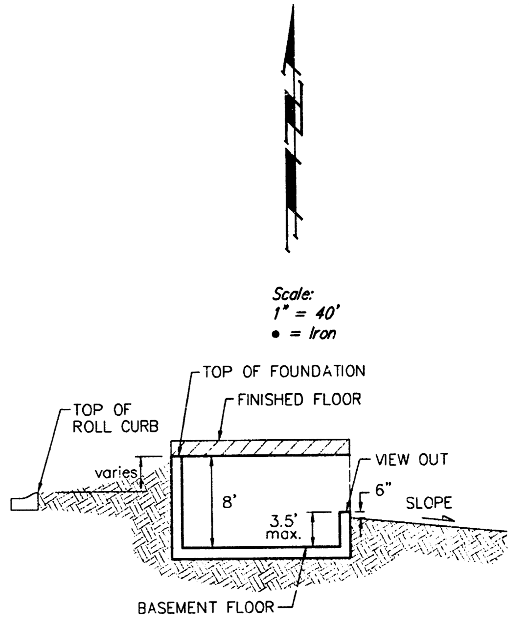
TYPICAL VIEW OUT NO SCALE
