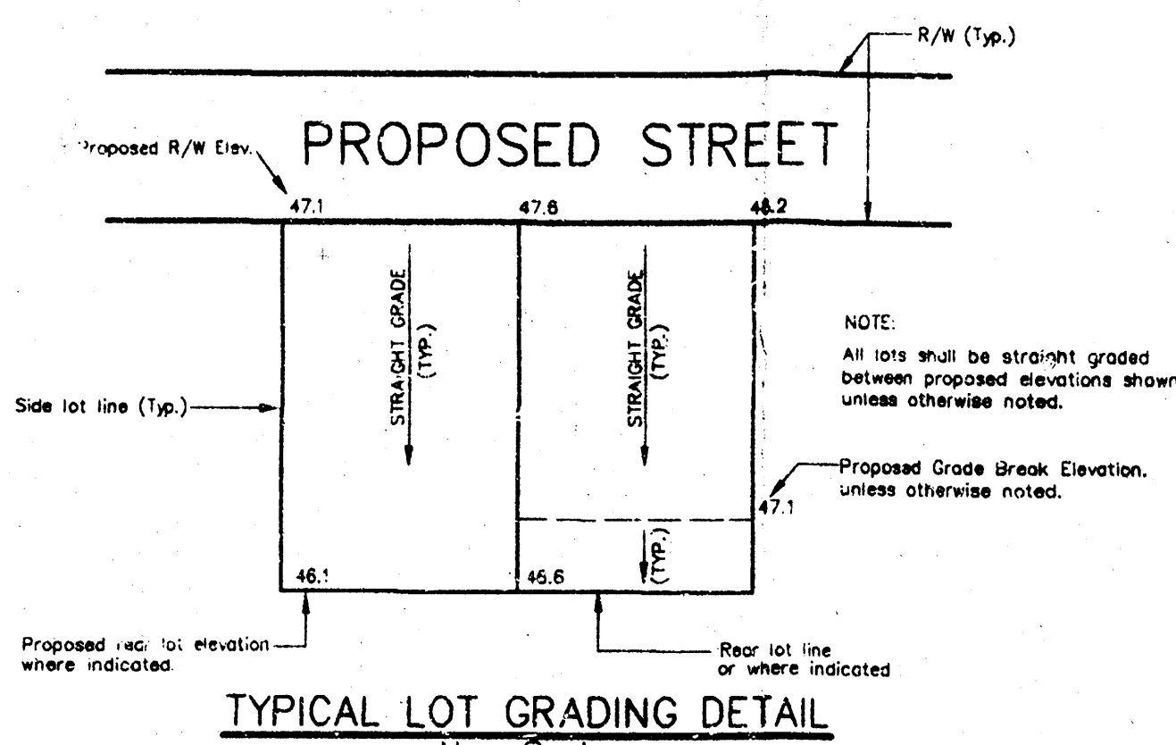
TYPICAL LOT GRADING DETAIL NO SCALE
