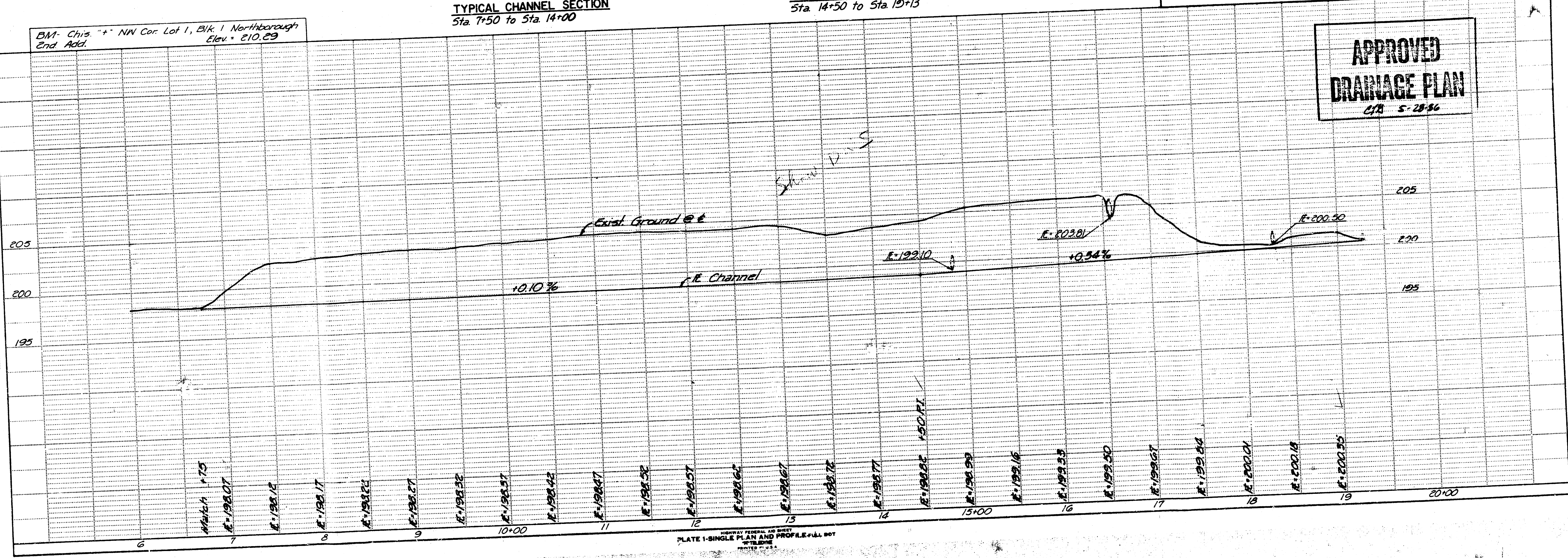
TYPICAL CHANNEL SECTION Sta. 14+50 to Sta. 19+13
