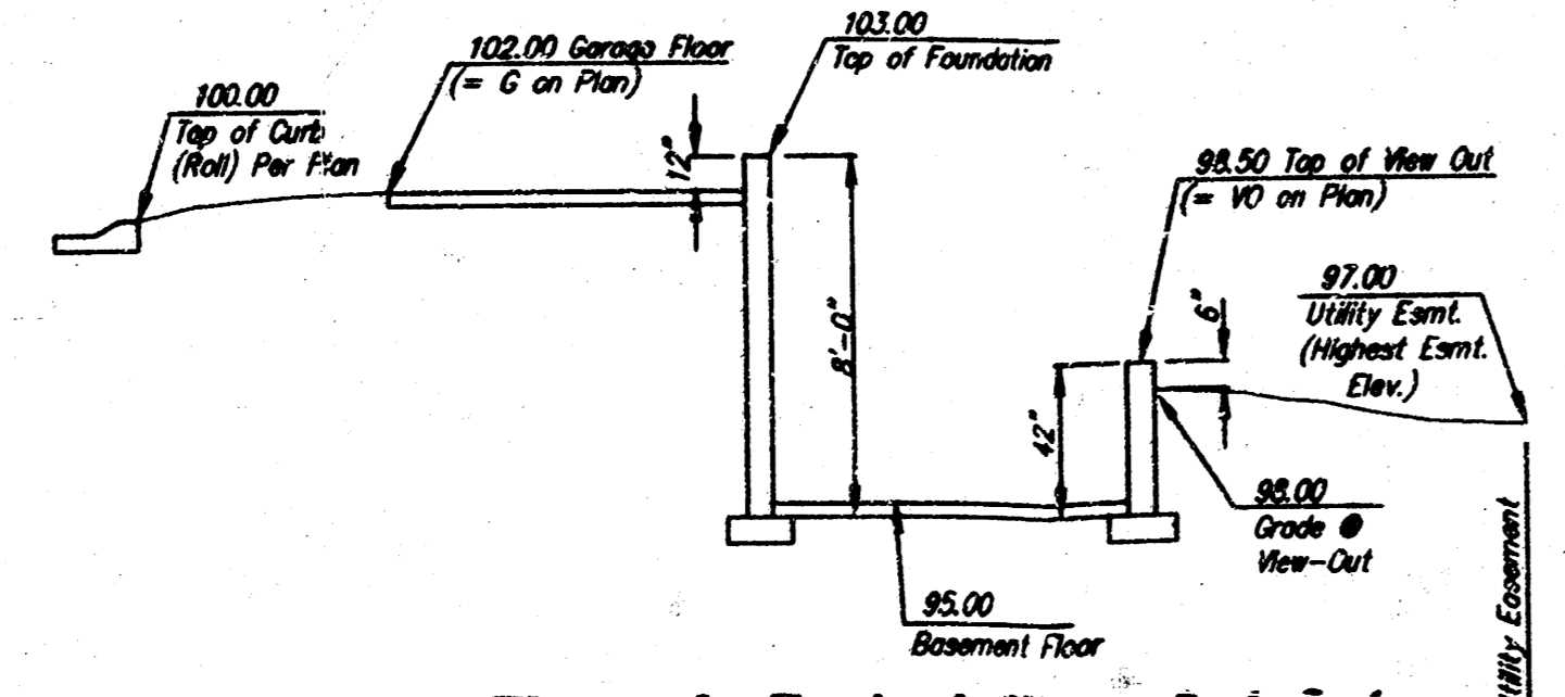
Section Through Typical View-Out Lot 100.00 Assumed T.C. Elevation for section
