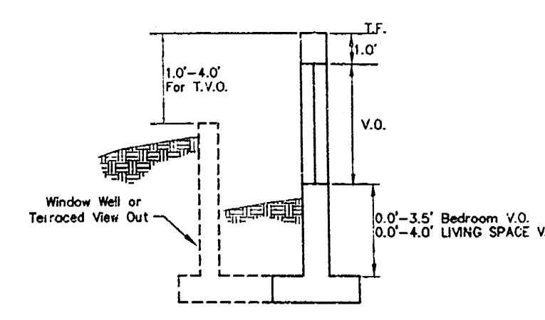
VIEW OUT & TERRACED VIEW OUT DETAIL
