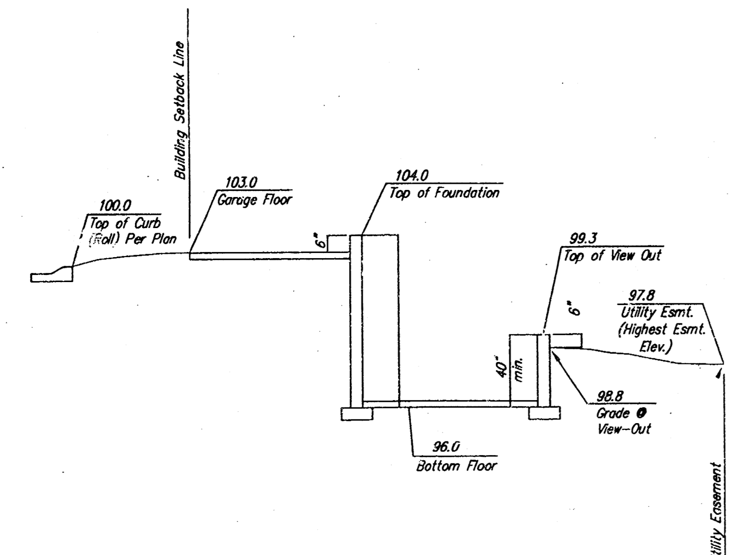
Section Through Typical View-Out Lot
