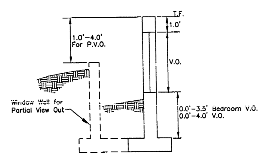
VIEW OUT & PARTIAL VIEW OUT DETAIL
