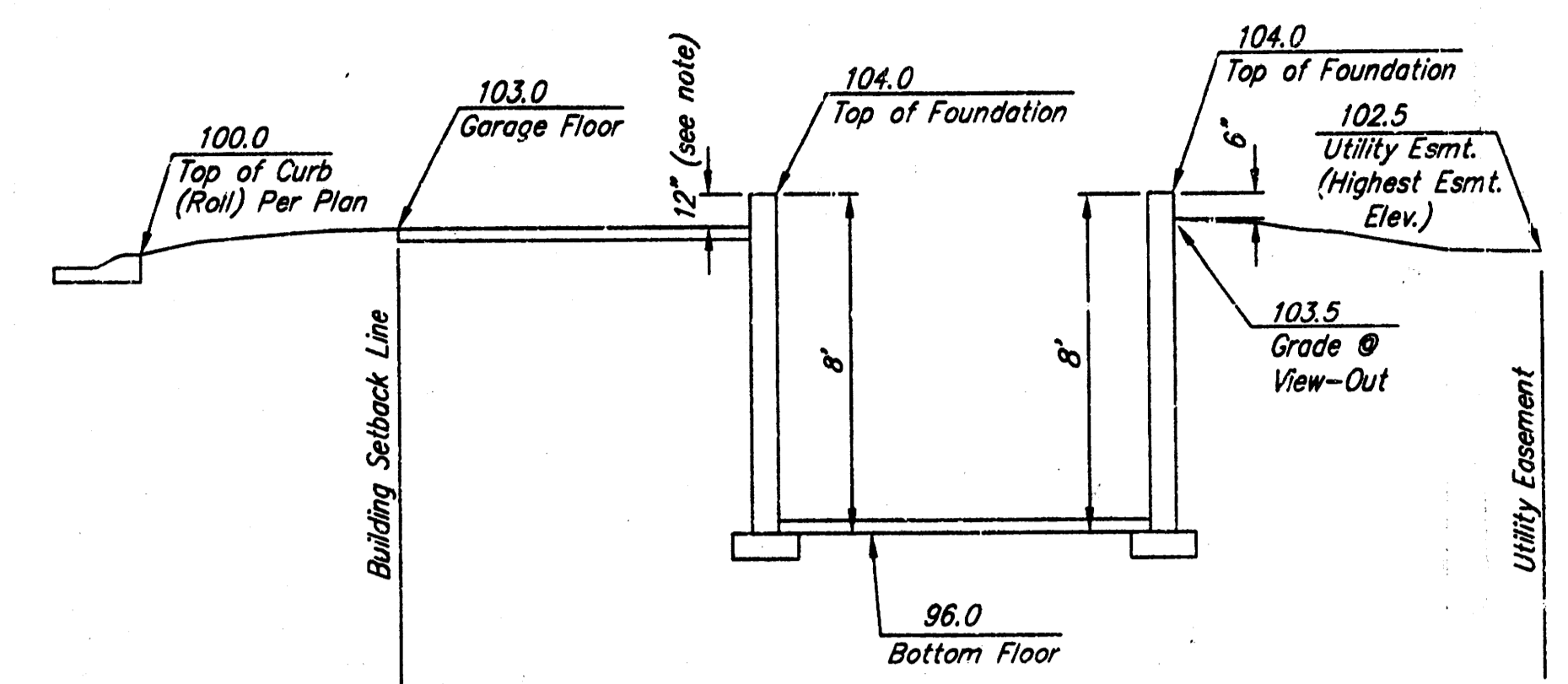
Section Through Typical Full Basement
