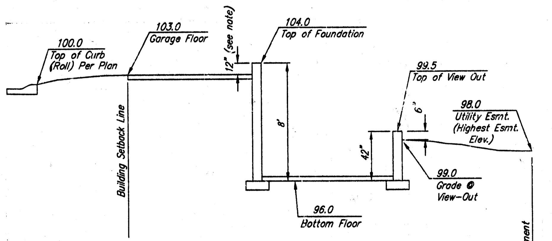
Section Through Typical View-Out Lot
