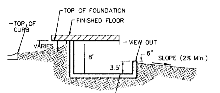
TYPICAL VIEW OUT DETAIL NO SCALE
