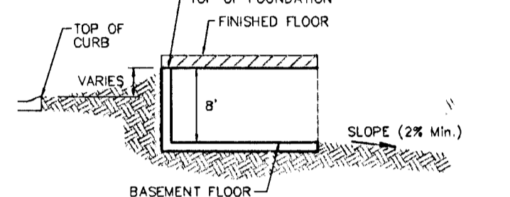
TYPICAL WALK OUT DETAIL NO SCALE
