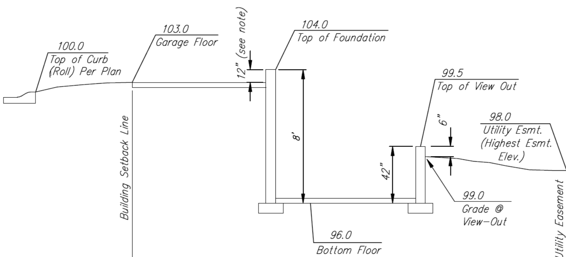
Section Through Typical View-Out Lot
