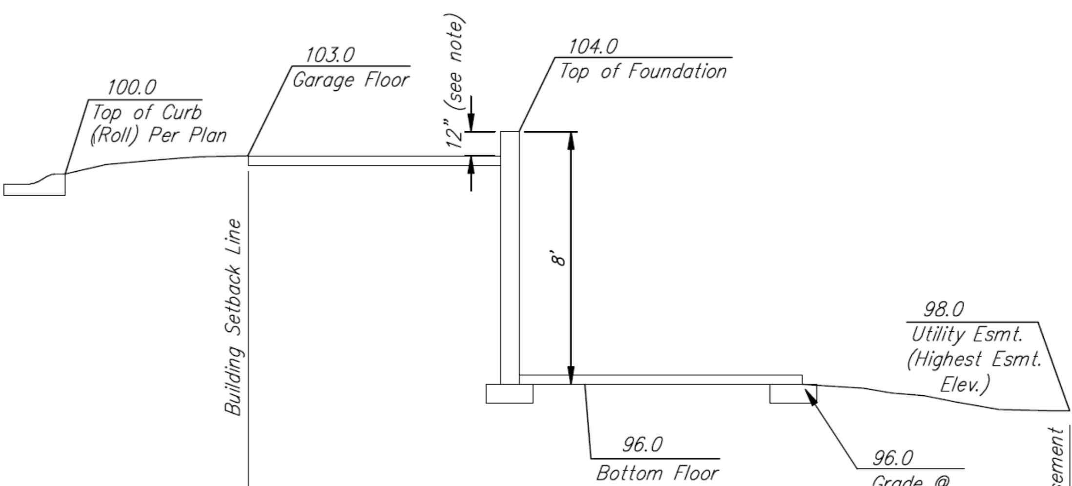
Section Through Typical Walk-Out Lot
