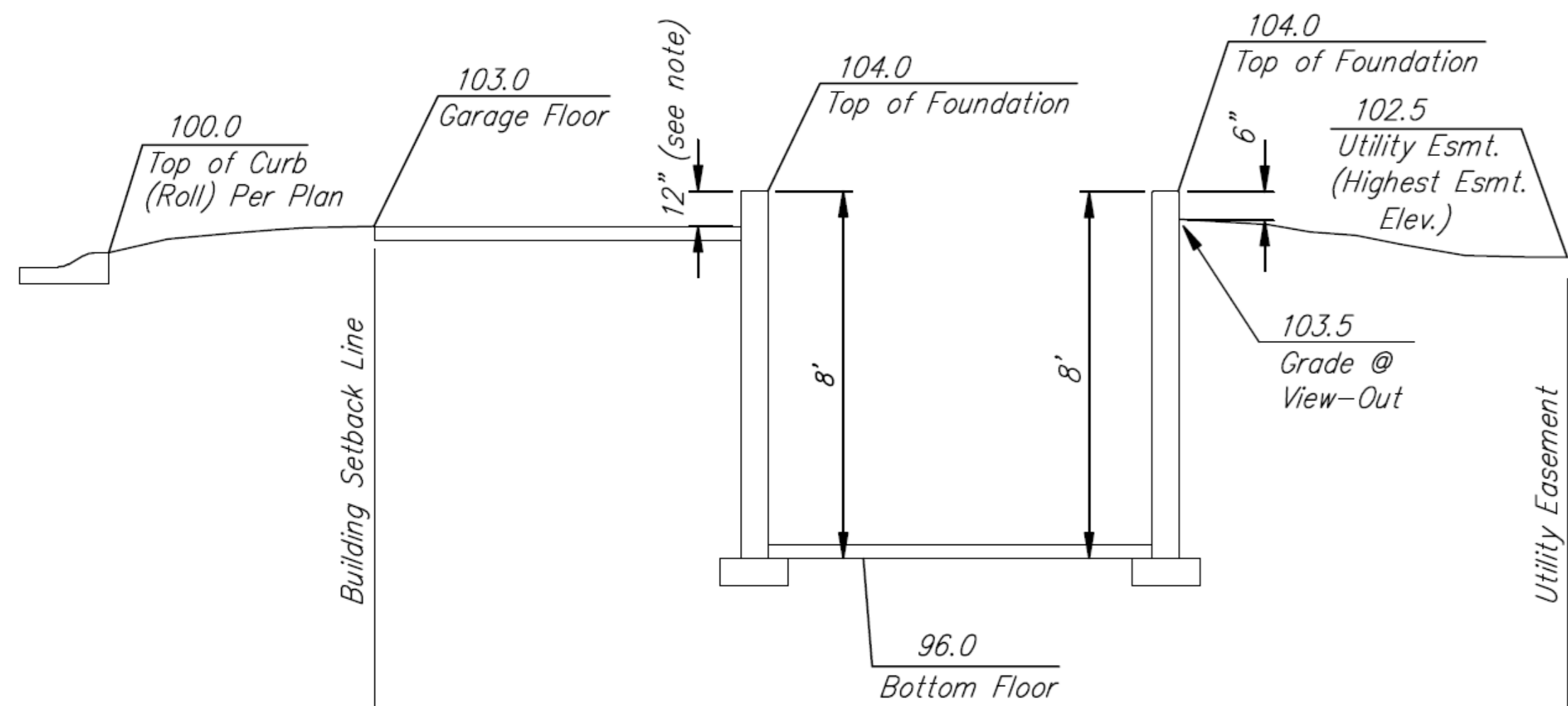
Section Through Typical Full Basement
