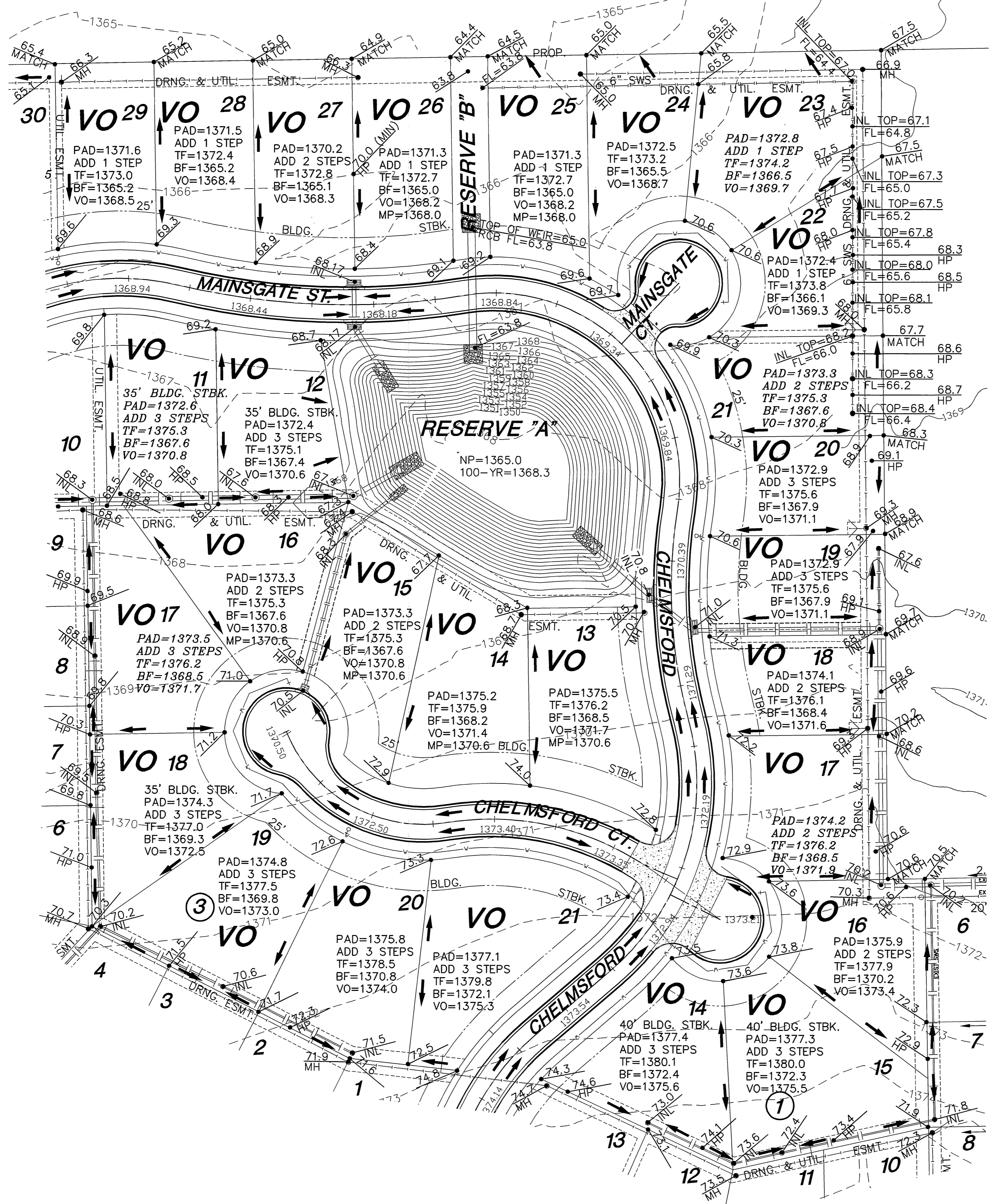
VIEW OUT & TERRACED VIEW OUT DETAIL
