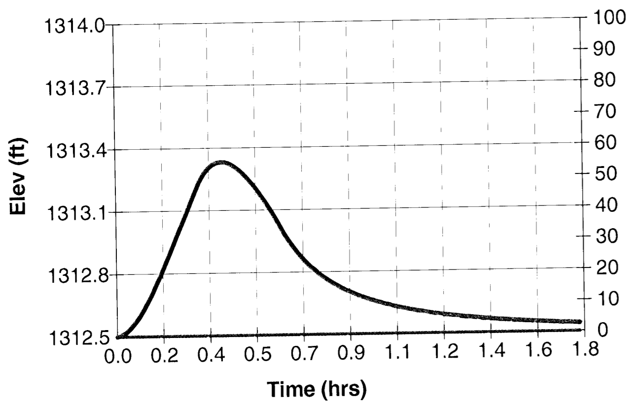
2 - Reservoir - 100 Yr - Max. El. = 1313.33 ft
