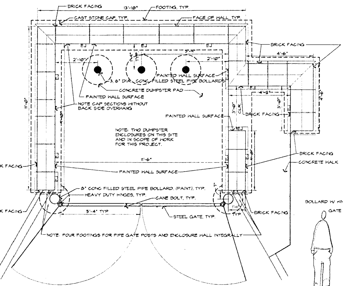
PLAN - DUMPSTER ENCLOSURE NOT TO SCALE
