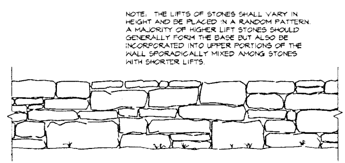
ELEVATION - TYPICAL DRY STONE WALL / TREE WELL NOT TO SCALE
