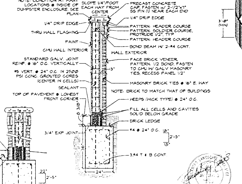
WALL SECTION NOT TO SCALE
