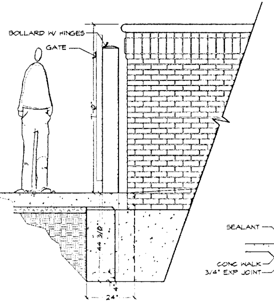
ELEVATION - DUMPSTER ENCLOSURE NOT TO SCALE
