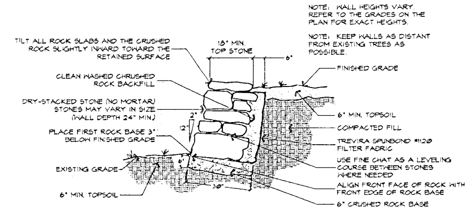
SECTION - DRY STONE RETAINING WALL / TREE WELL NOT TO SCALE
