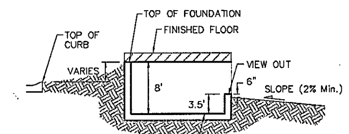
TYPICAL VIEW OUT DETAIL NO SCALE
