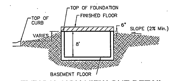
TYPICAL NON-VIEW OUT DETAIL NO SCALE
