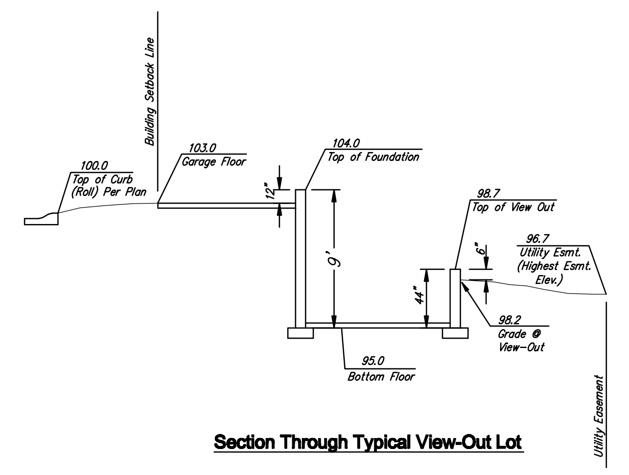
Section Through Typical Walk-Out Lot
