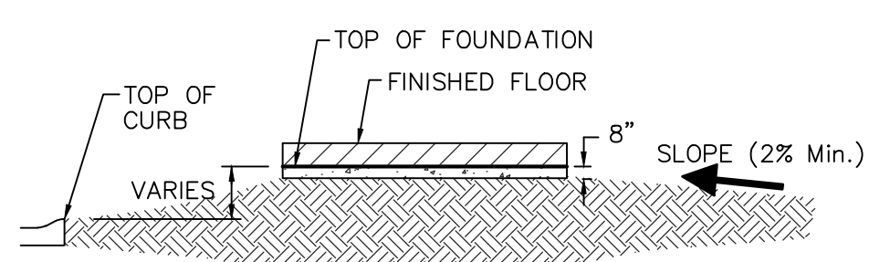
TYPICAL SLAB FOUNDATION DETAIL NO SCALE
