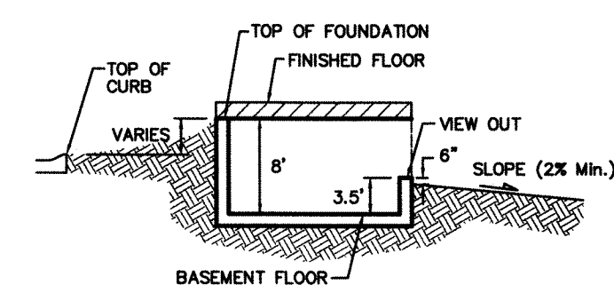
TYPICAL VIEW OUT DETAIL NO SCALE
