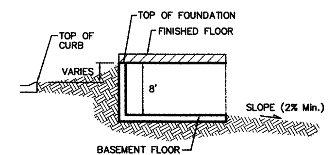
TYPICAL WALK OUT DETAIL NO SCALE
