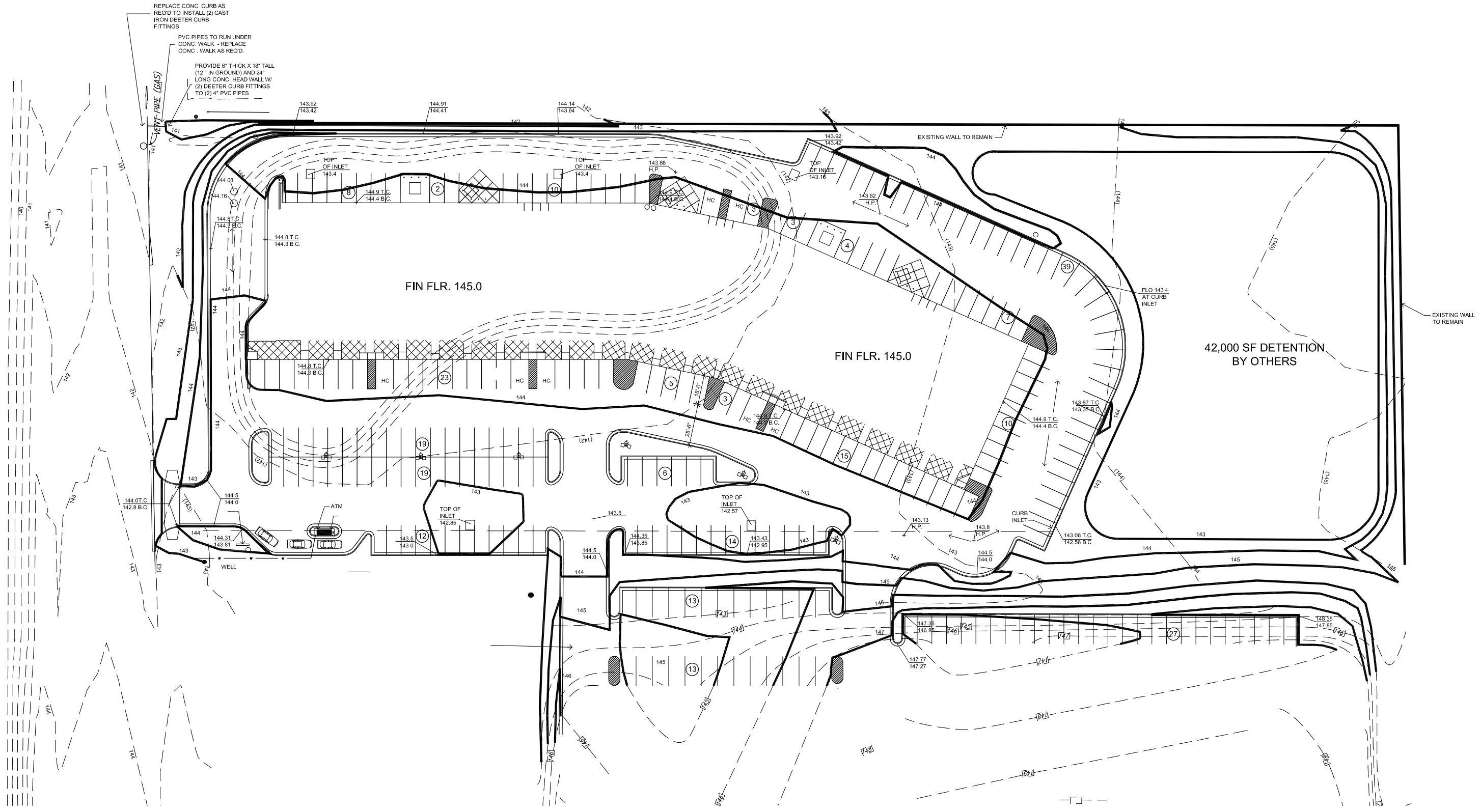
GRADING PLAN 0 30'
