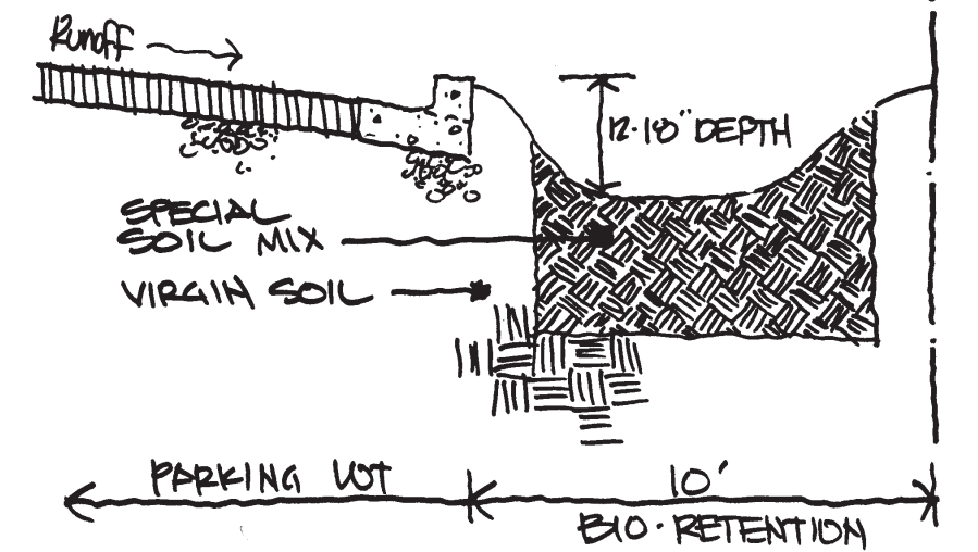
Typical Cross-Section Thru Bio-Retention Swale
