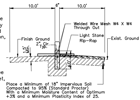
SECTION B-B No Scale
