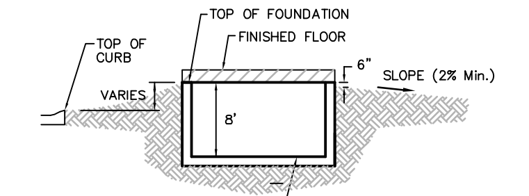
TYPICAL NON-VIEW OUT DETAIL
