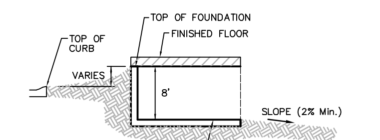
TYPICAL WALK OUT DETAIL
