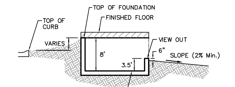
TYPICAL VIEW OUT DETAIL
