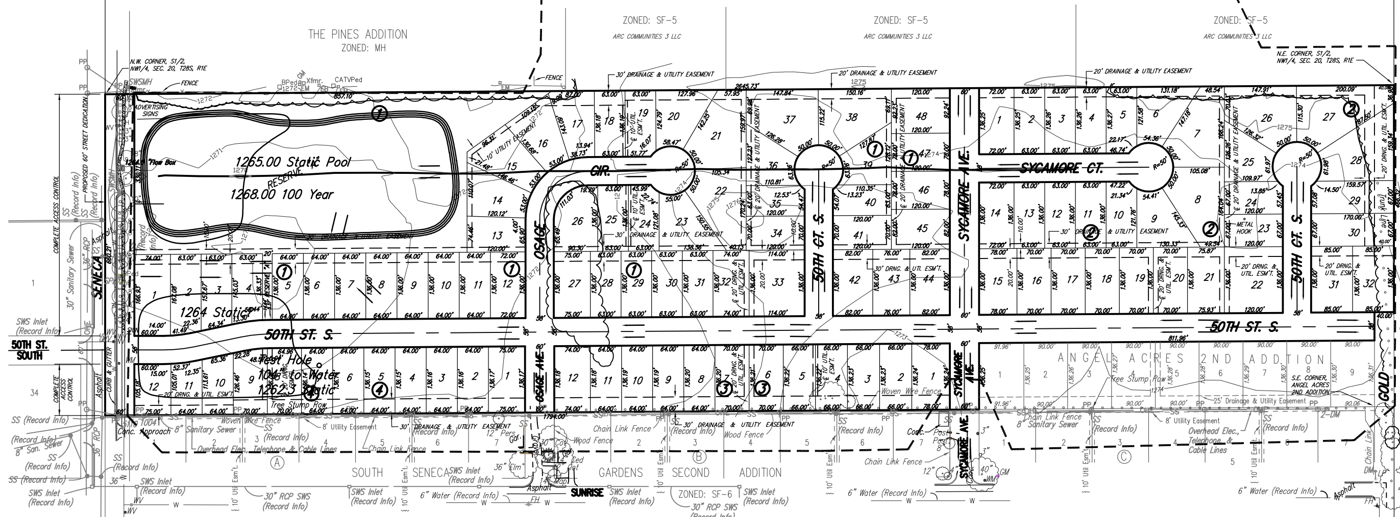
MAP 2 - RESULTING DRAINAGE AREA TO DETENTION POND
